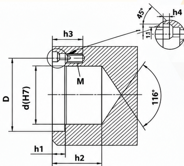
SECTION VIEW
